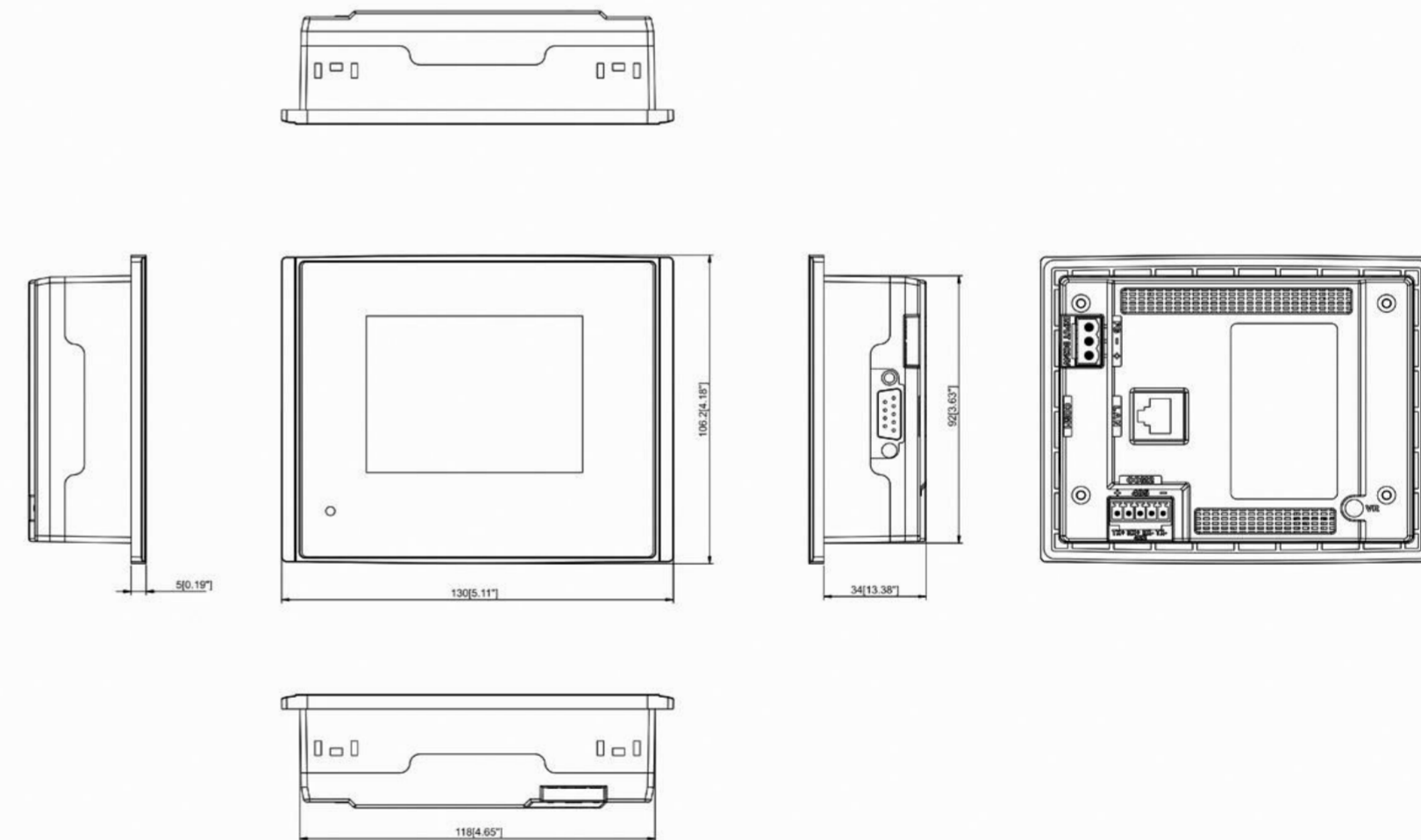
Panel Cut Out Dimensions: 119 x 93 mm
