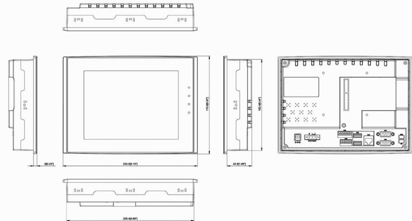
Panel Cut Out Dimensions: 221.4 x 164.4 mm
